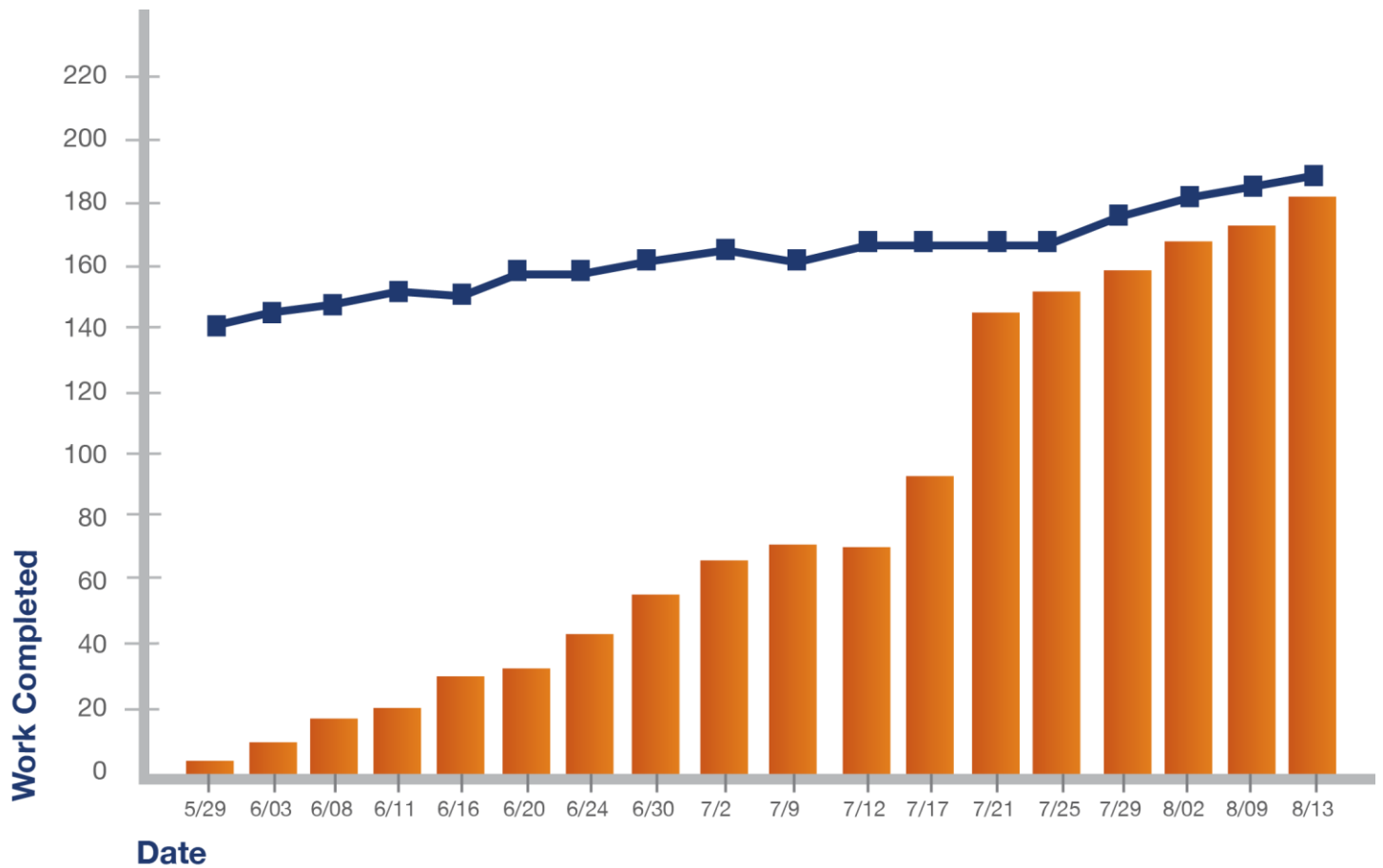
Figure 6 Typical Burn-Up Chart
